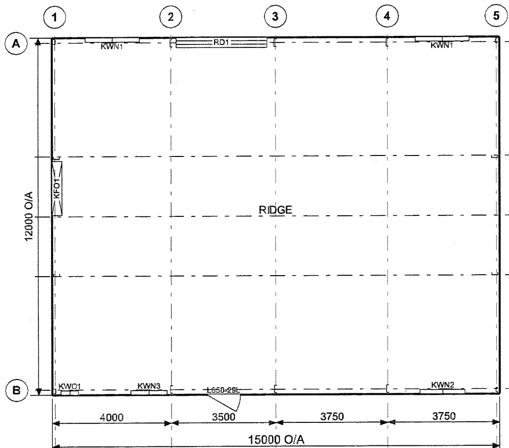
FRAME ROOF PLAN
